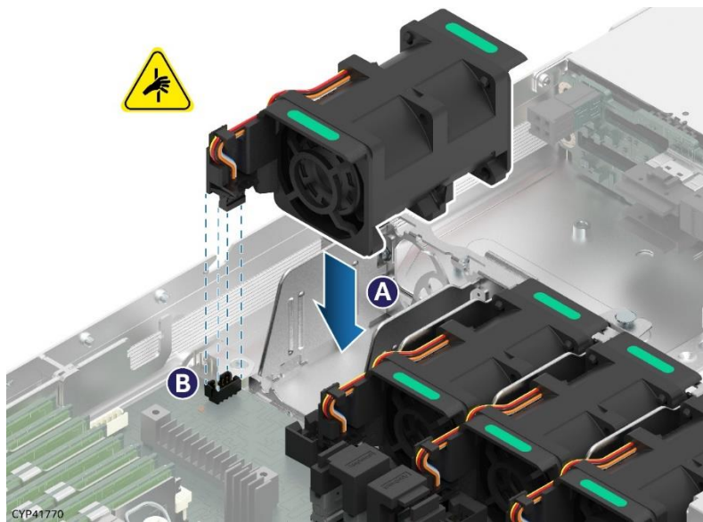
Figure 78. Individual Fan Installation
