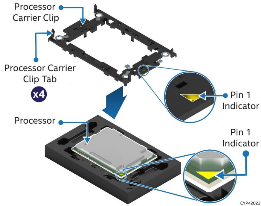
Figure 87. Installing Processor Carrier Clip onto Processor – Part 1
