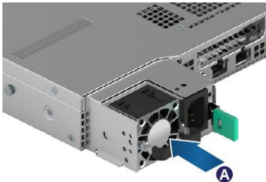
Figure 82. Power Supply Installation
