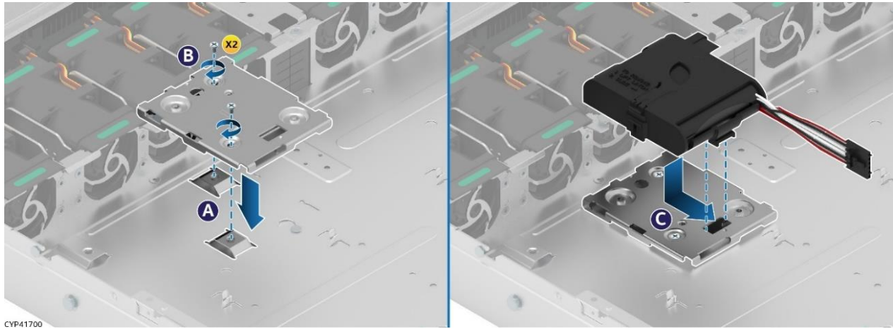
Figure 61. Intel® RMFBU Mounting Bracket Installation
