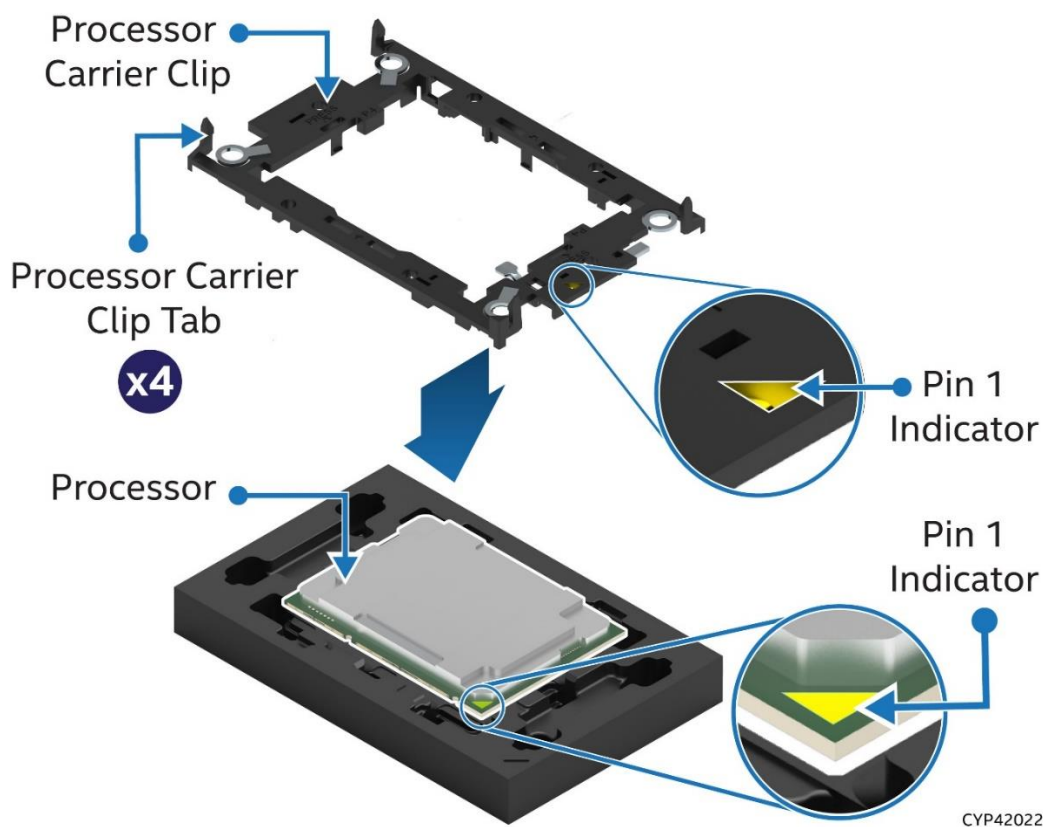
Figure 7. Installing Processor Carrier Clip onto Processor – Part 1
