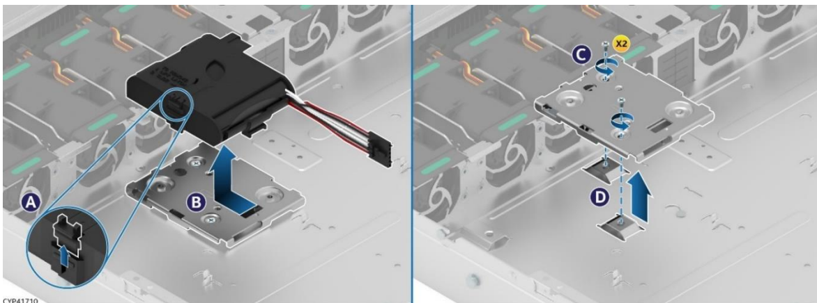
Figure 62. Intel® RMFBU Mounting Bracket Removal - Chassis
