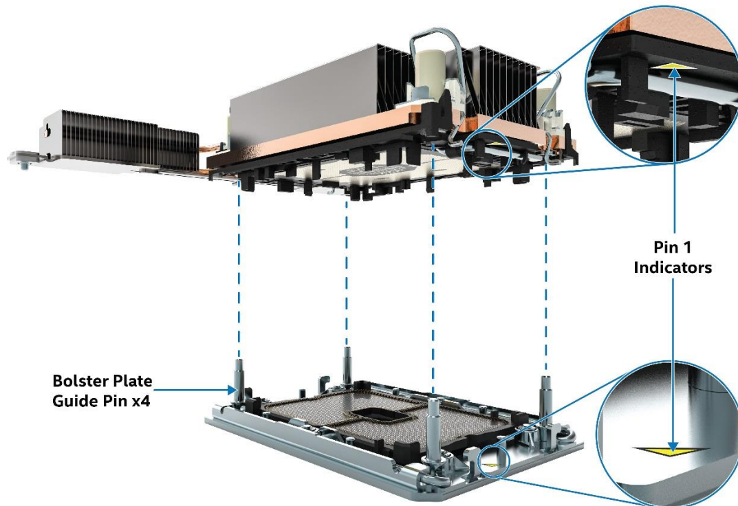
Figure 93. PHM Alignment with Socket Assembly
