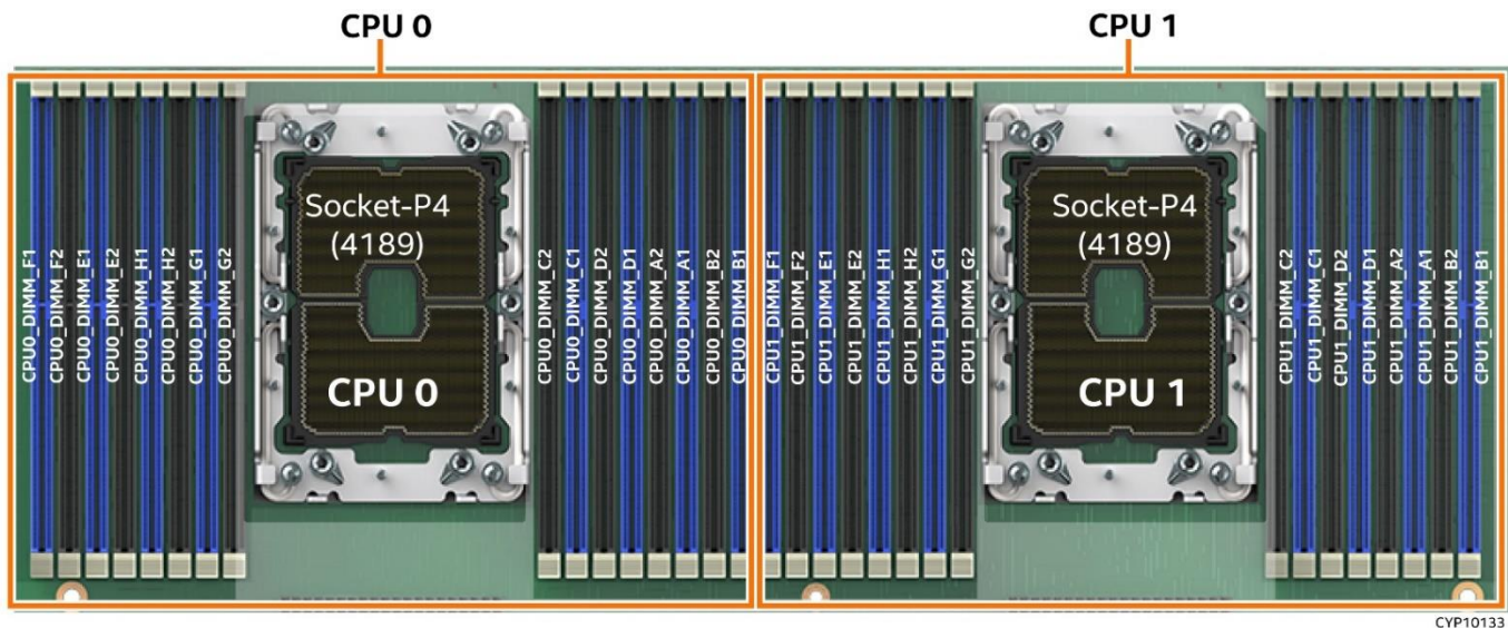
Figure 114. Intel® Server System M50CYP1UR Family Memory Slot Layout
