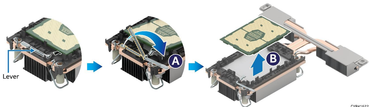
Figure 85. Processor Removal from PHM Assembly
