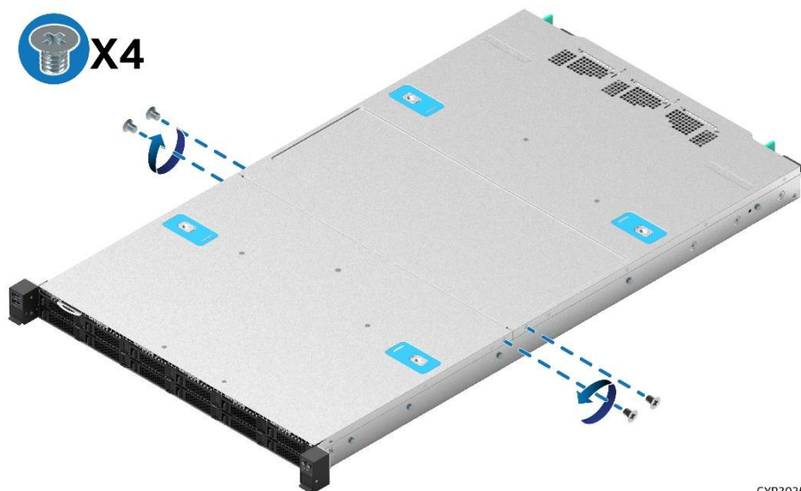
Figure 19. System Top Cover Panel Shipping Screws
