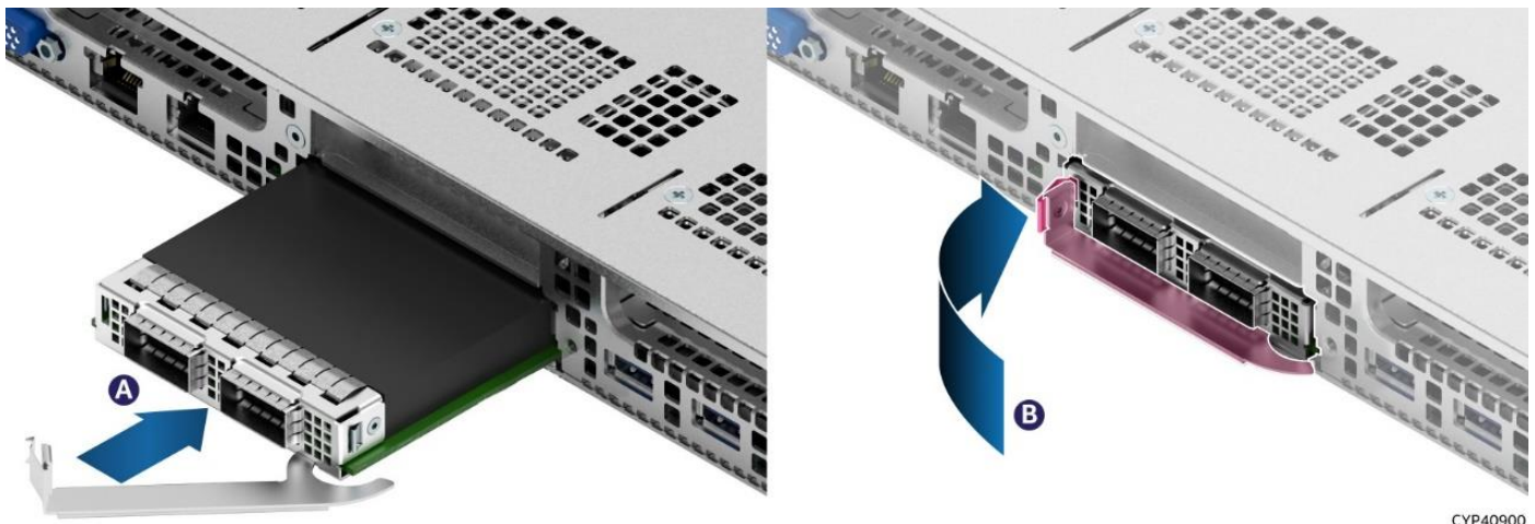
Figure 44. OCP* Adapter with Ejector Latch Installation
