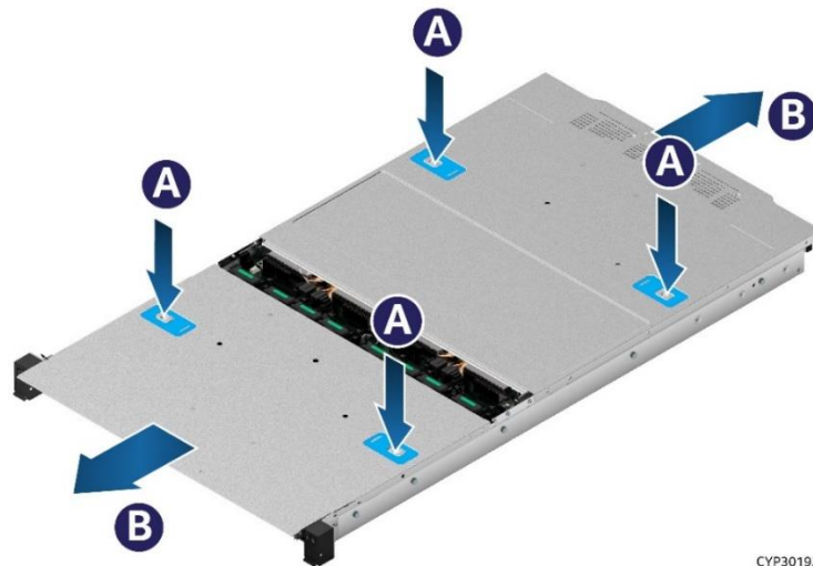
Figure 75. System Cover Removal
