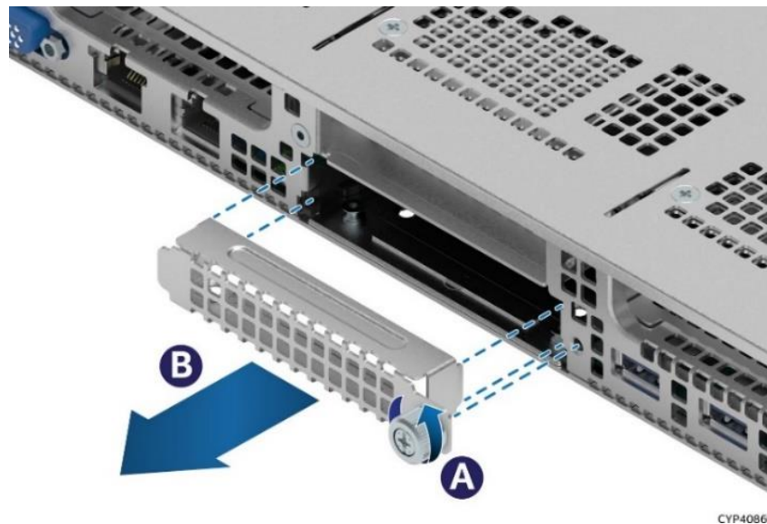
Figure 40. OCP* Adapter Bay Filler Removal
