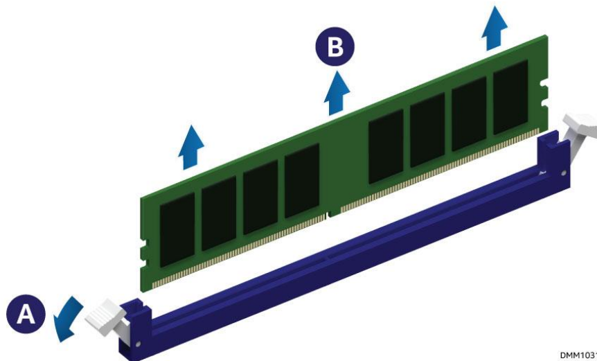
Figure 79. Memory Module Removal
