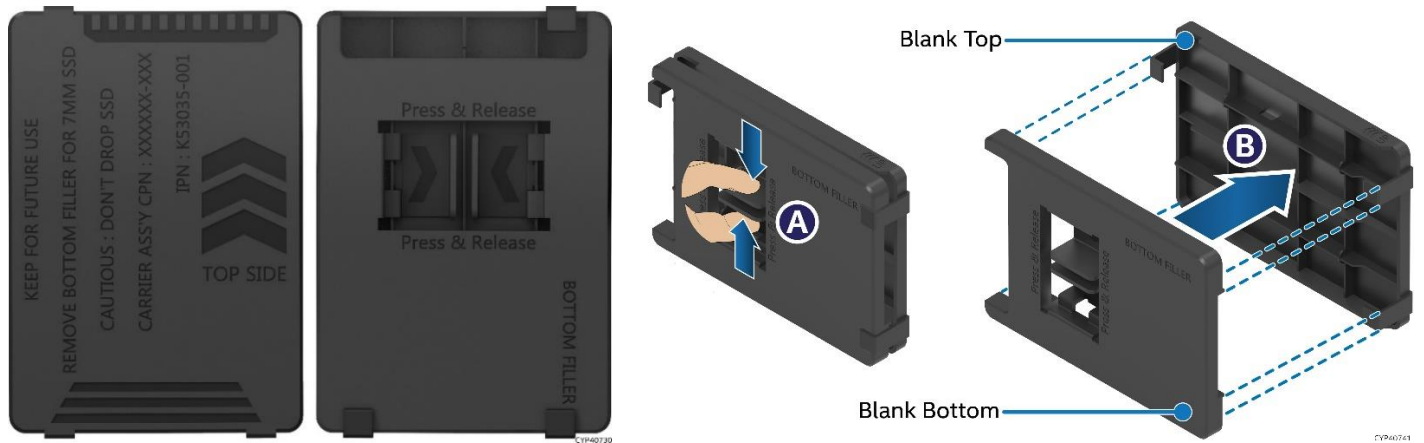
Figure 99. Separating Top and Bottom Parts of Drive Blank
