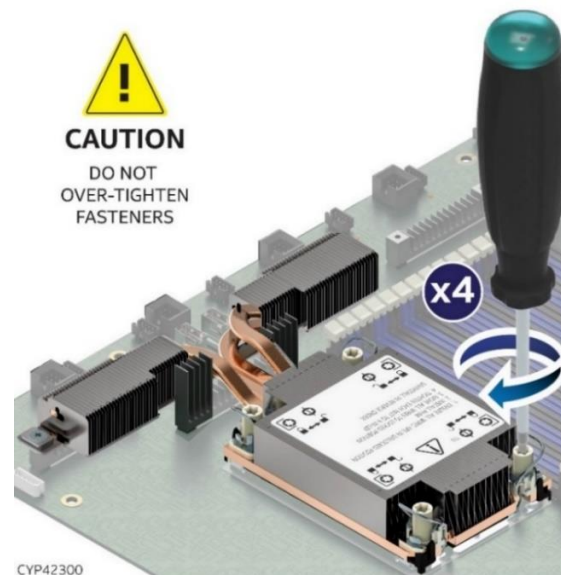
Figure 15. Tighten Heat Sink Extension Fasteners
