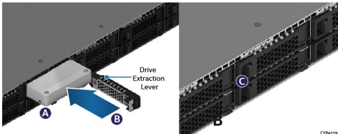
Figure 37. 2.5" 15 mm Drive Installation
