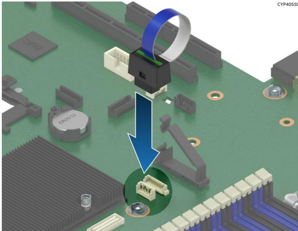
Figure 53. Intel® VROC Key Insertion
