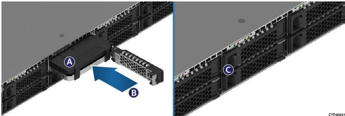
Figure 35. 2.5" 7 mm Drive Installation
