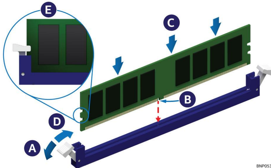
Figure 17. Memory Module Installation
