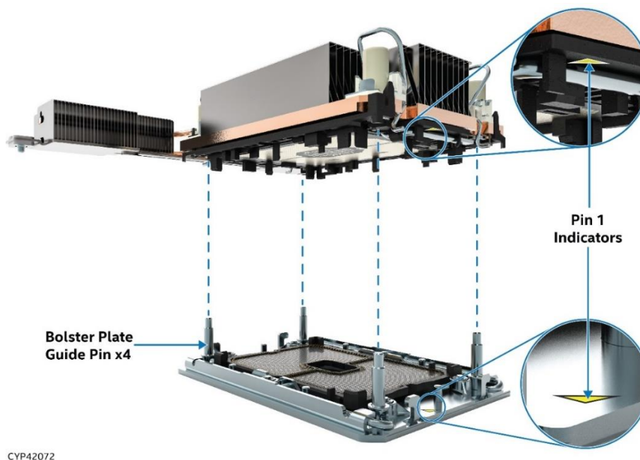
Figure 13. PHM Alignment with Socket Assembly
