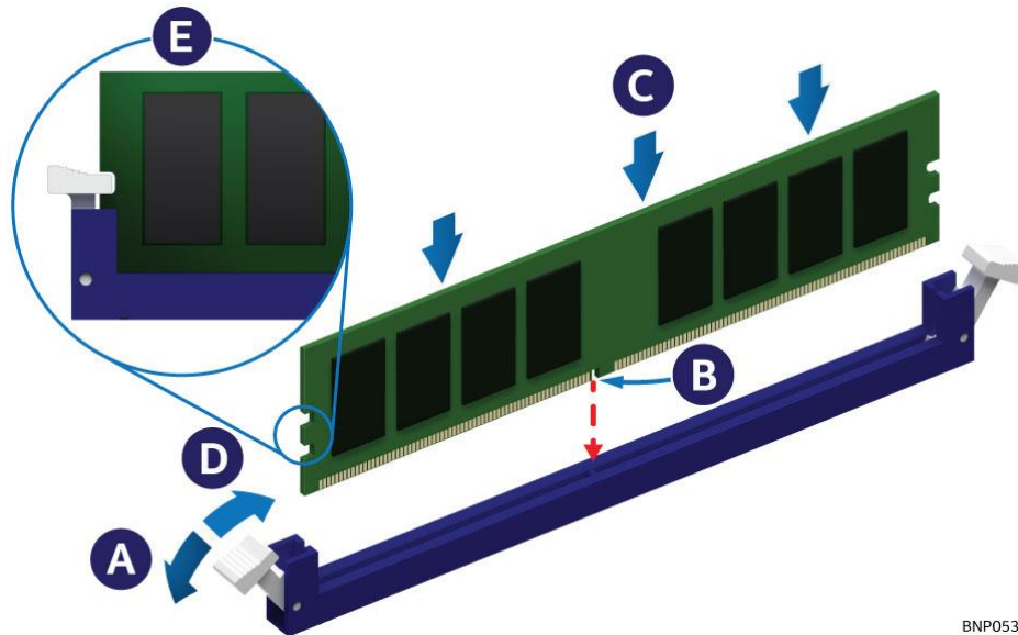
Figure 80. Memory Module Installation
