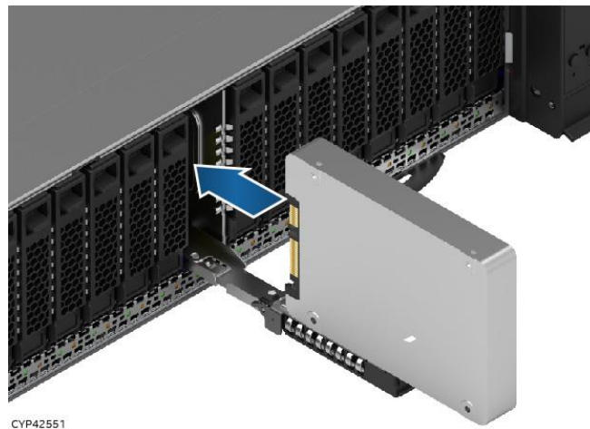
Figure 36. 2.5" 15 mm Drive Outside Chassis, Ready for Installation
