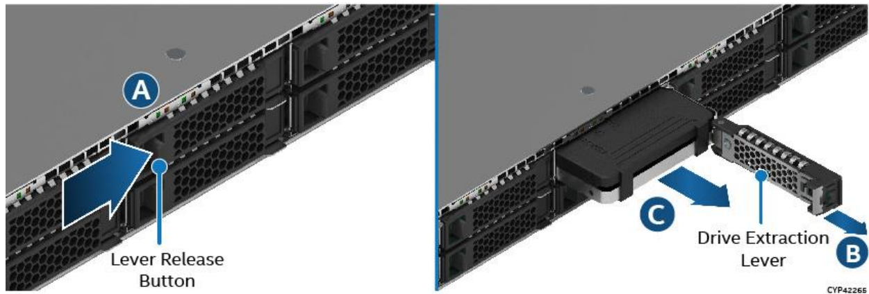
Figure 38. 2.5" 7 mm Drive Removal
