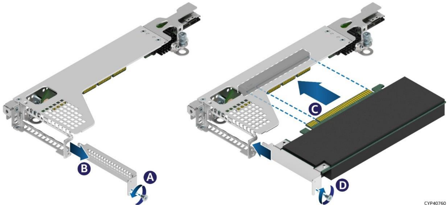
Figure 29. PCIe* Add-In Card Installation for Riser Card on Riser Slot #2
