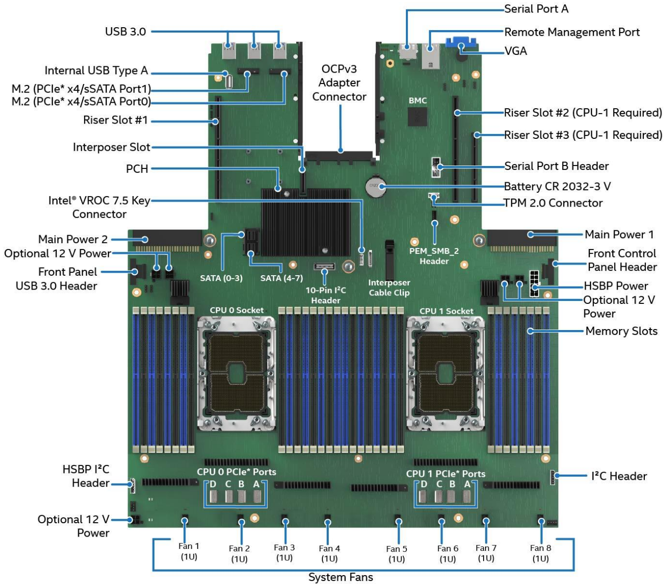
Figure 69. Intel® Server Board M50CYP2SB1U Component / Feature Identification
