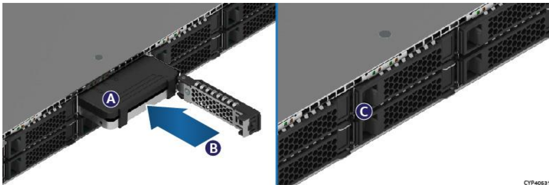
Figure 102. 2.5" 7 mm Drive Installation
