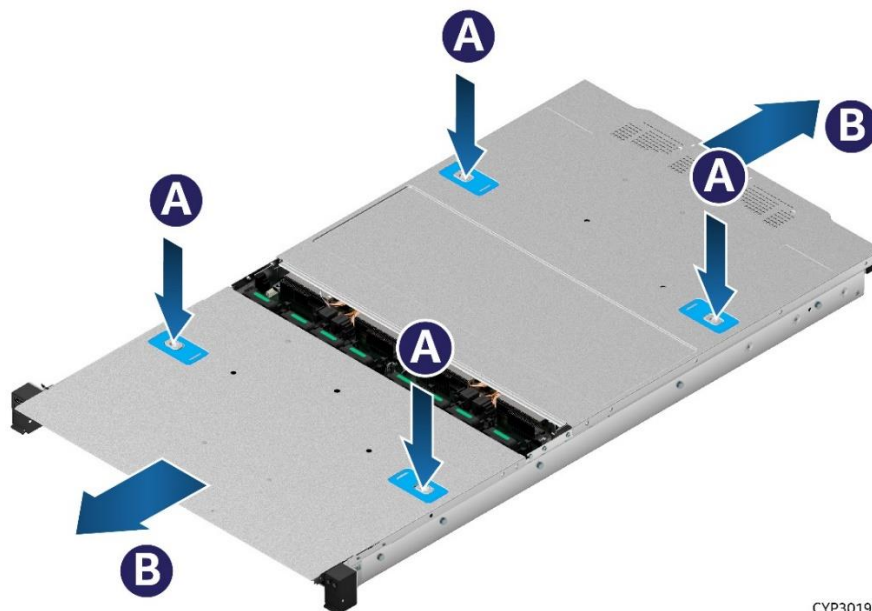
Figure 3. System Cover Removal
