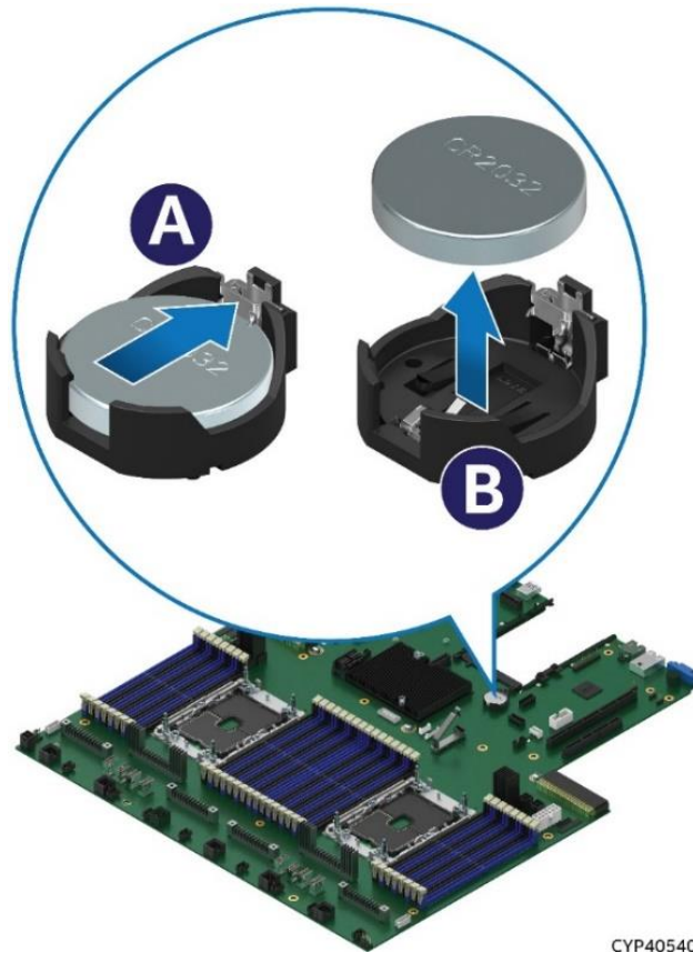
Figure 110. Replacing the System Battery
