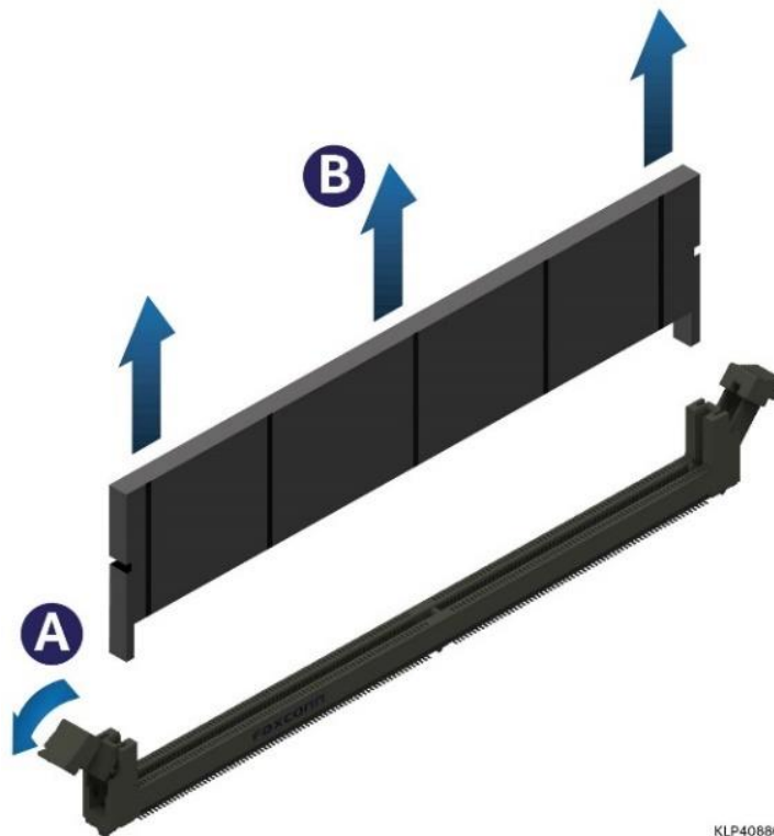
Figure 16. DIMM Blank Removal
