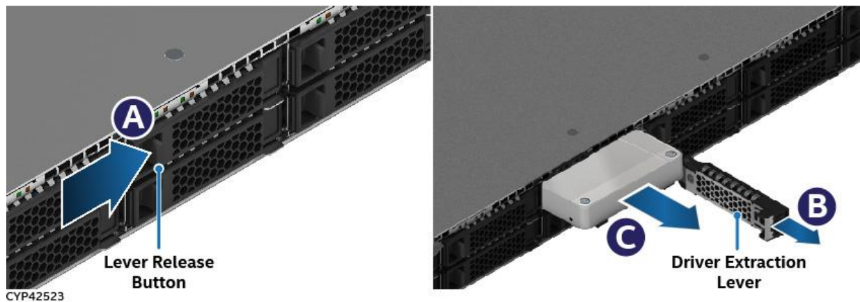
Figure 39. 2.5" 15 mm Drive Removal
