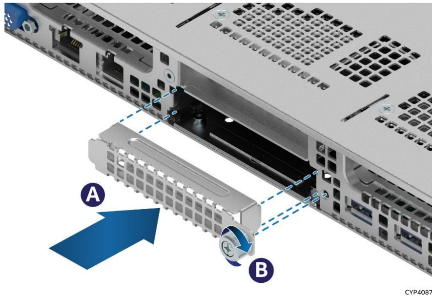
Figure 41. OCP* Adapter Bay Filler Installation
