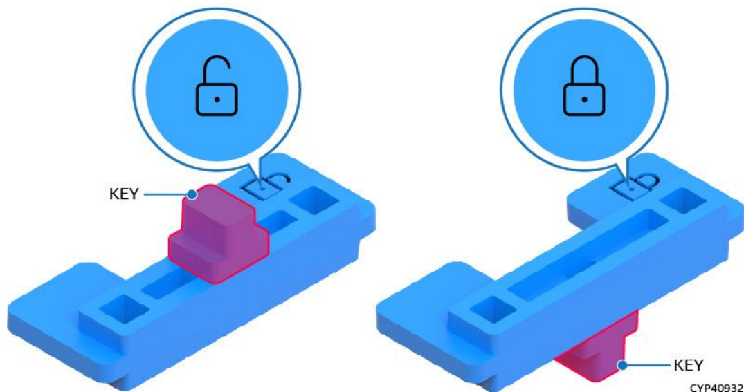
Figure 46. Internal Lock with Unlock and Lock Orientation
