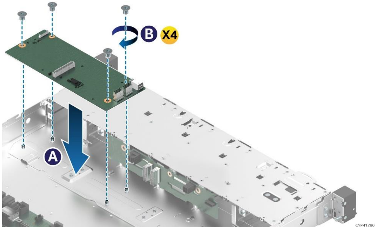
Figure 55. SAS Interposer Card Installation
