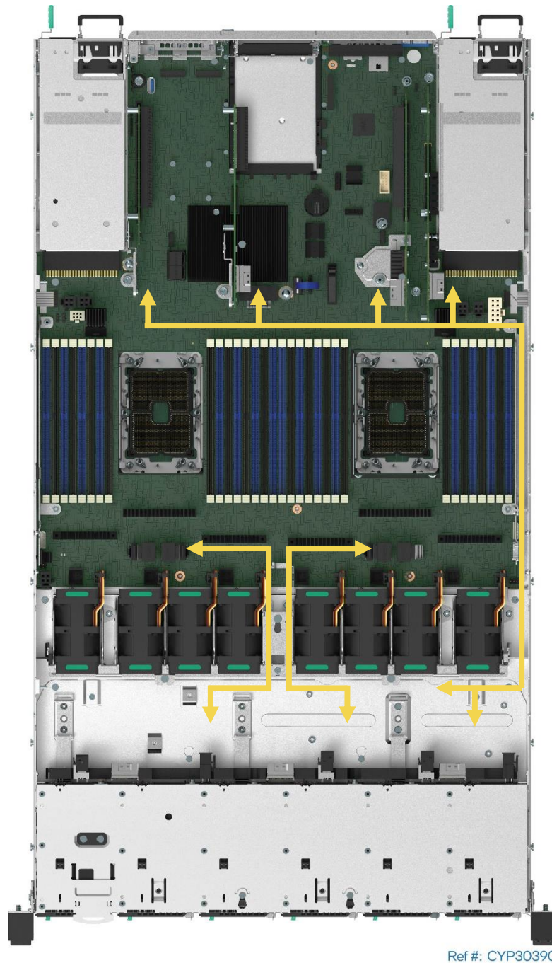
Figure 109. System Cable Routing Channels
