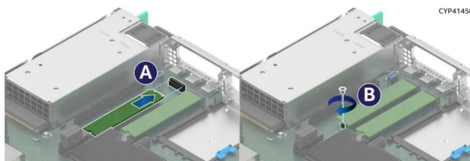
Figure 50. M.2 SSD Installation
